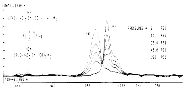
Figure 1. Infrared spectra of (PCy_3)_2Cr(CO)_3 under various pressures of H 2 . The peak at 1821 cm^{-1} due to (PCy_3)_2Cr(CO)_3 decreases as the band at 1836 cm^{-1} due to (PCy_3)_2Cr(CO)_3(H_2) increases. Spectra run at 25.0 °C in toluene.
